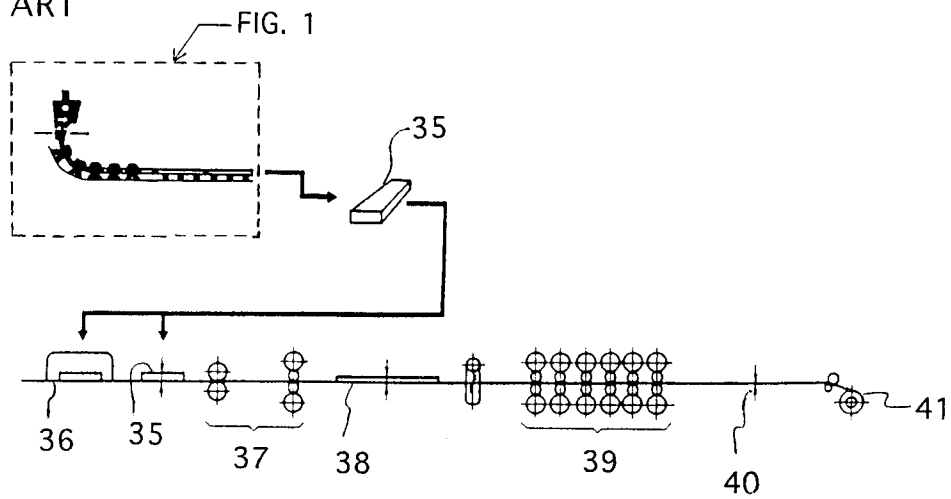
FIG. 2 PRIOR ART
