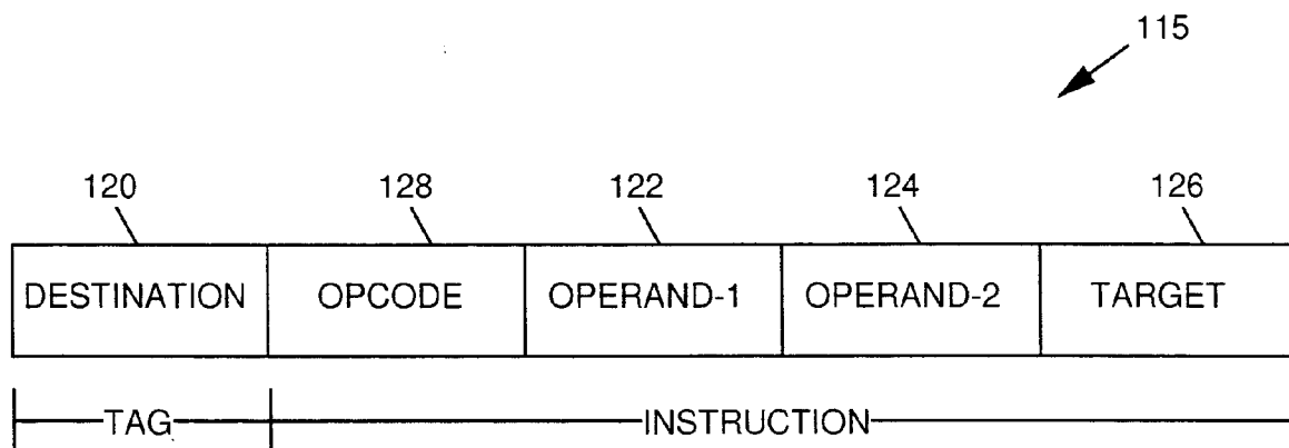
Second Example Instruction Format for Communications
