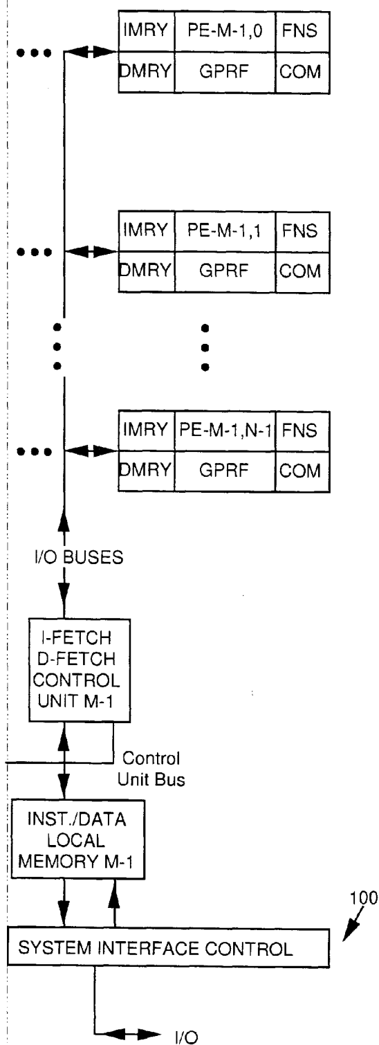
High Level Array Machine Organization Multiple Control Units
