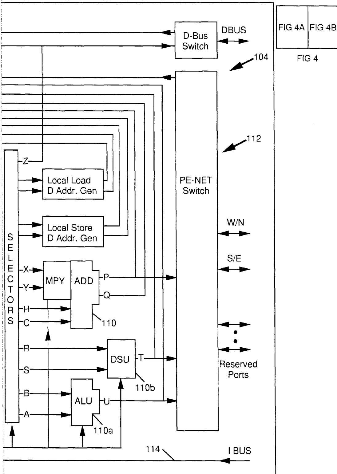
Single-PE (diagonal) Node Flow with Connection Interfaces
