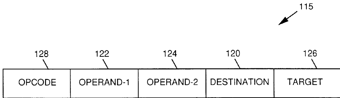
First Example Instruction Format for Communications
