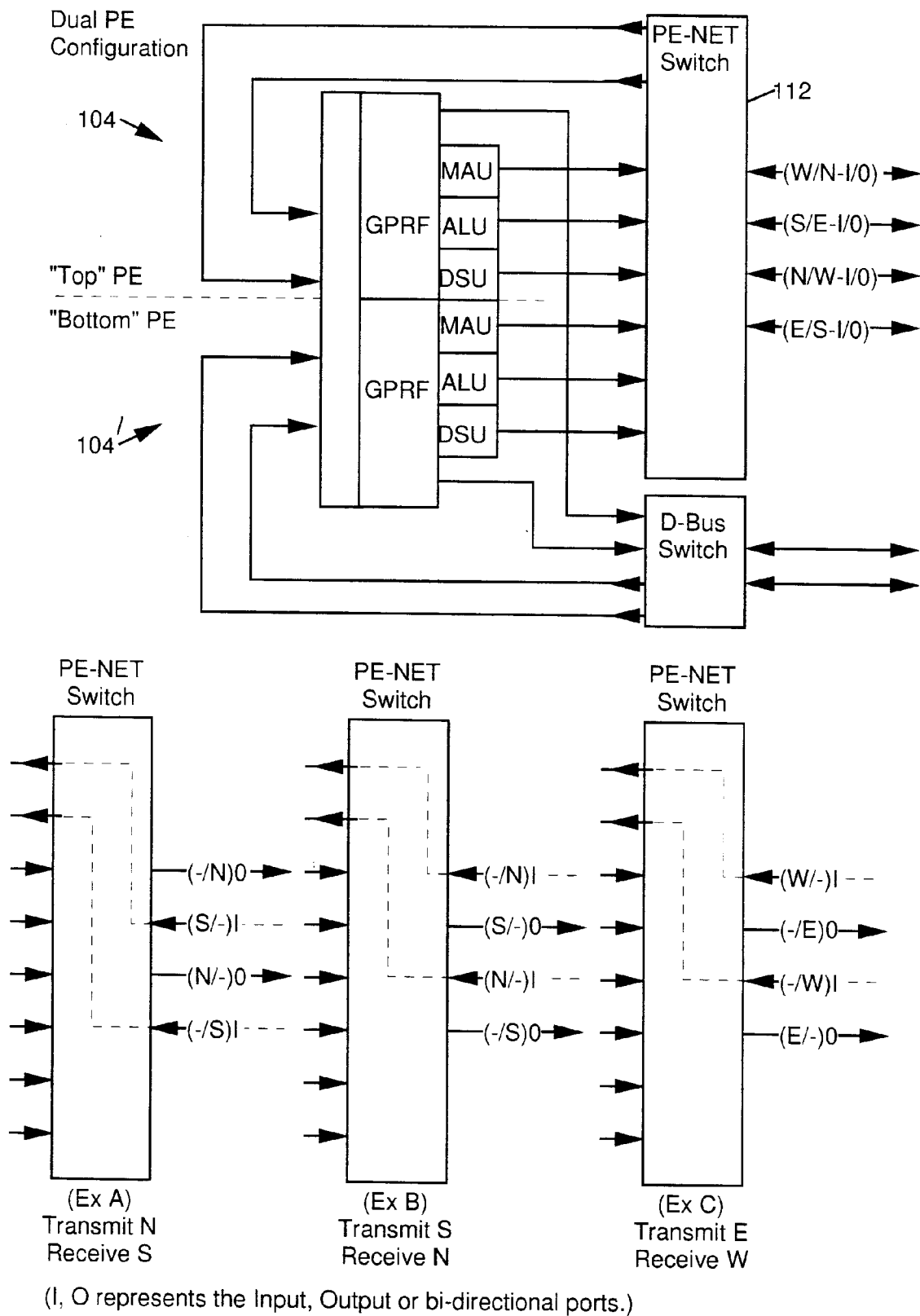
Nearest-Neighbor Communication Examples in a Dual-PE Node
