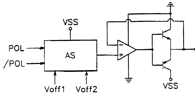
FIG.4 (Prior Art)
