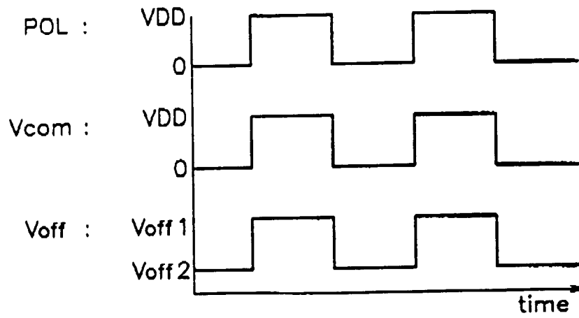
FIG.5(Prior Art)
