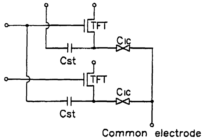
FIG.1 (Prior Art)
