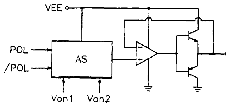
FIG.2 (Prior Art)
