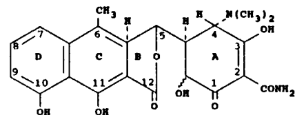
α- and β-Apooxytetracycline (α-APOTC, β-APOTC)
