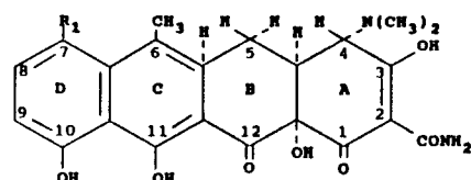
R 1 4-Epiplanhydrotetracycline (EATC) H 4-Epiplanhydrochlor-tetracycline (EACTC) Cl
