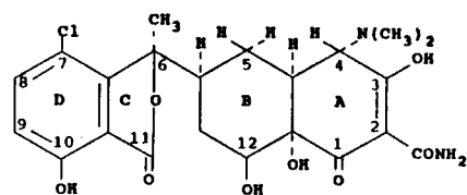
Isochlortetracycline (ISOCTC)
