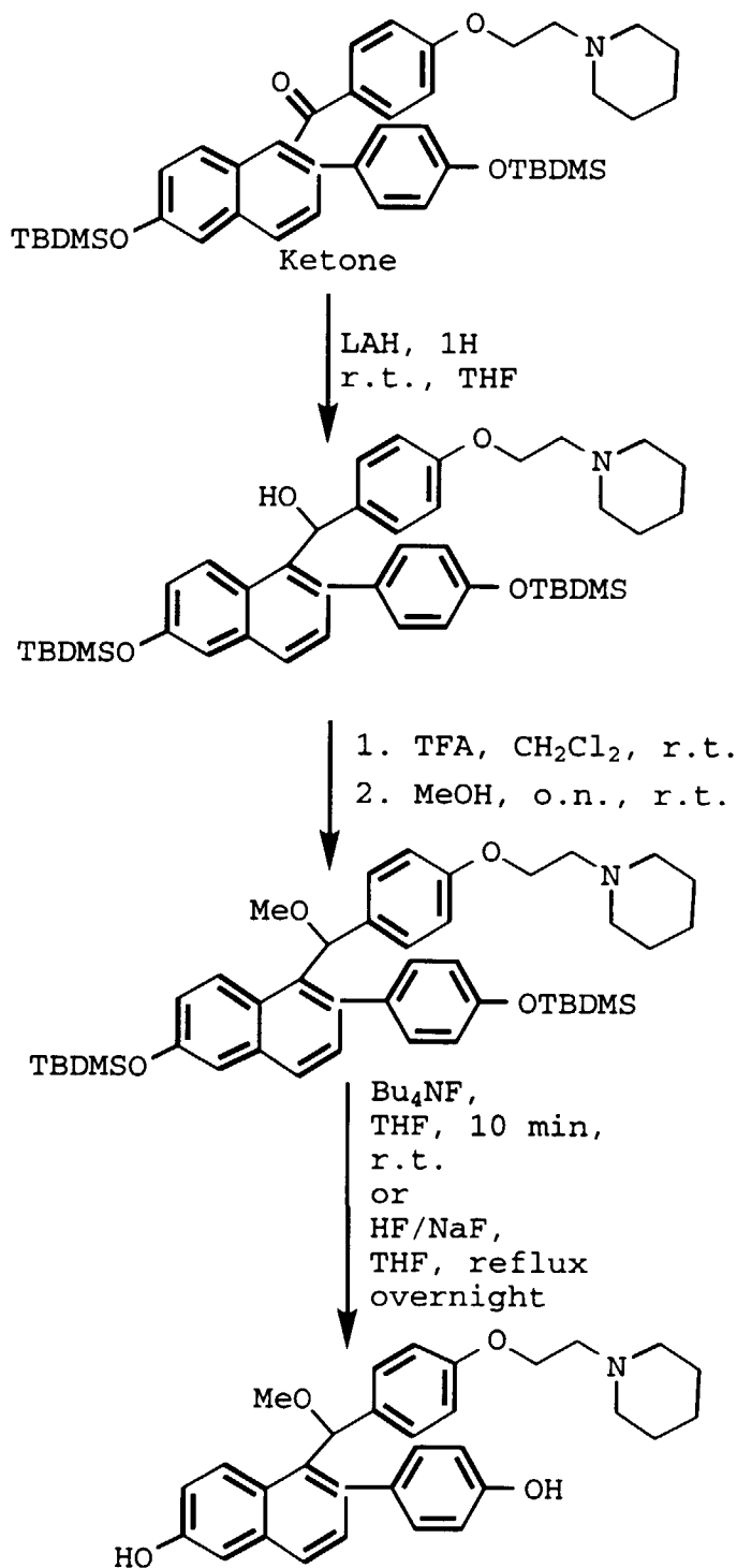
Scheme 1
