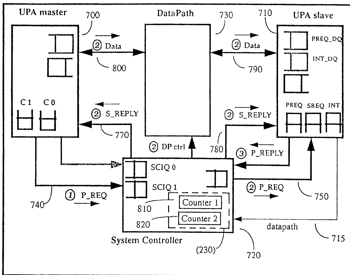
Slave Write Flow Control
