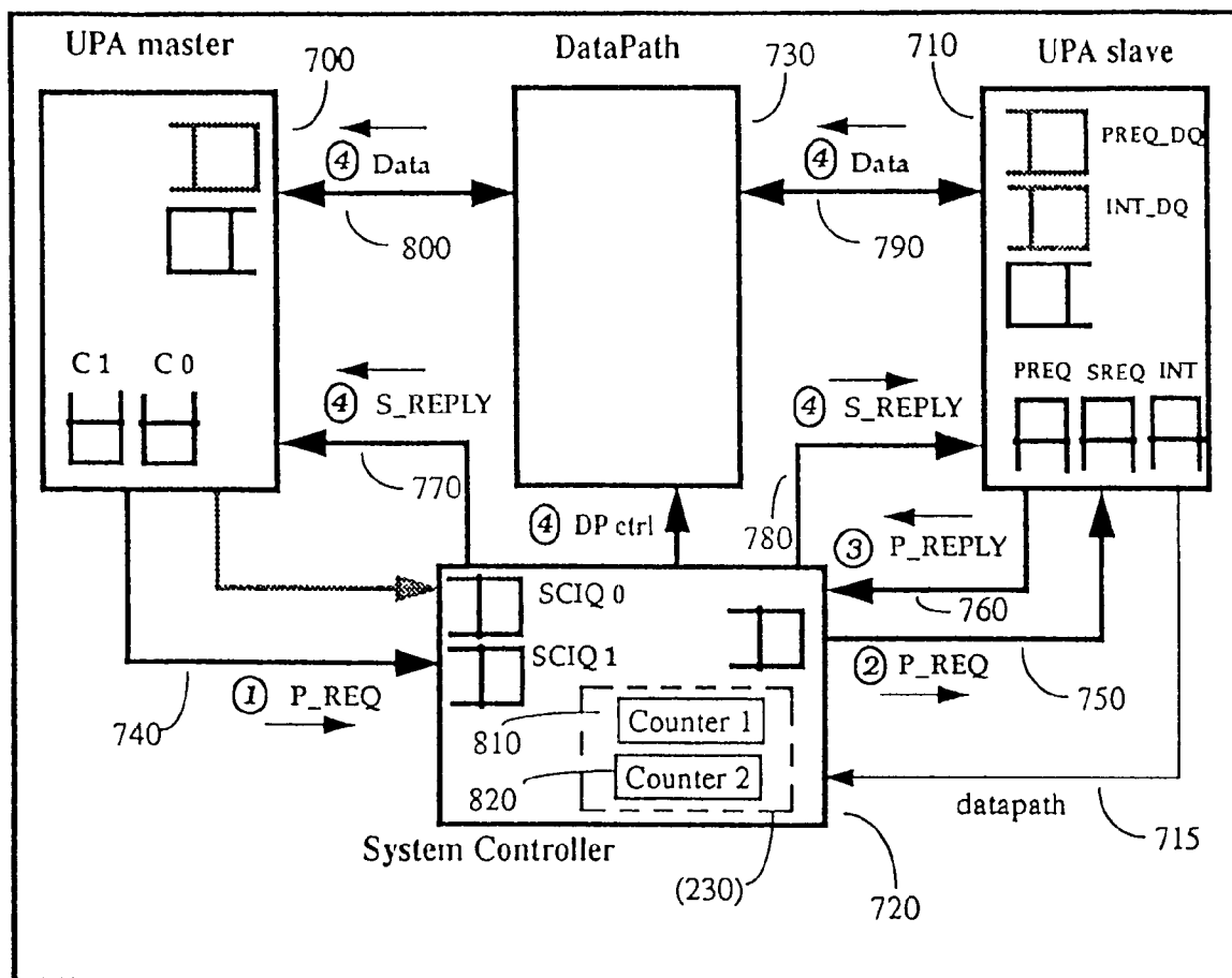
Slave Read Flow Control
