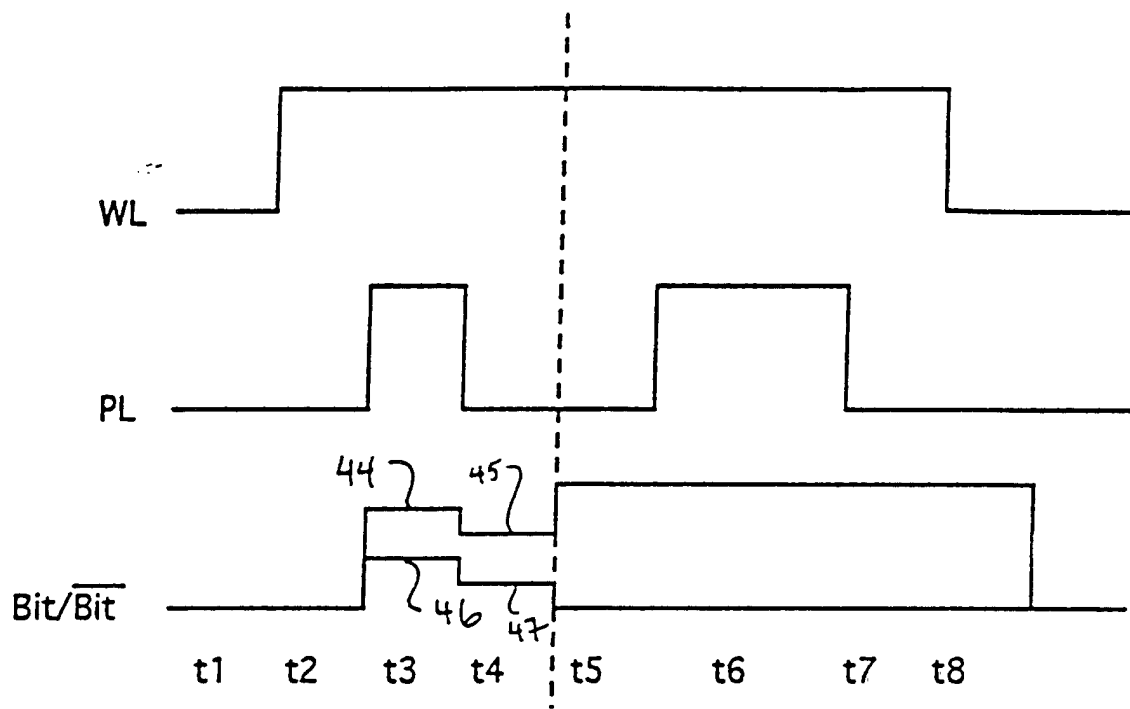
FIG. 3 Prior Art
