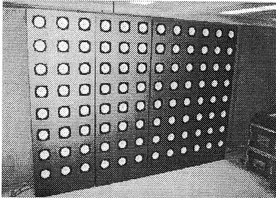
Virtual window constructed of 96 pieces of the loud speakers serving as the acoustic generators
