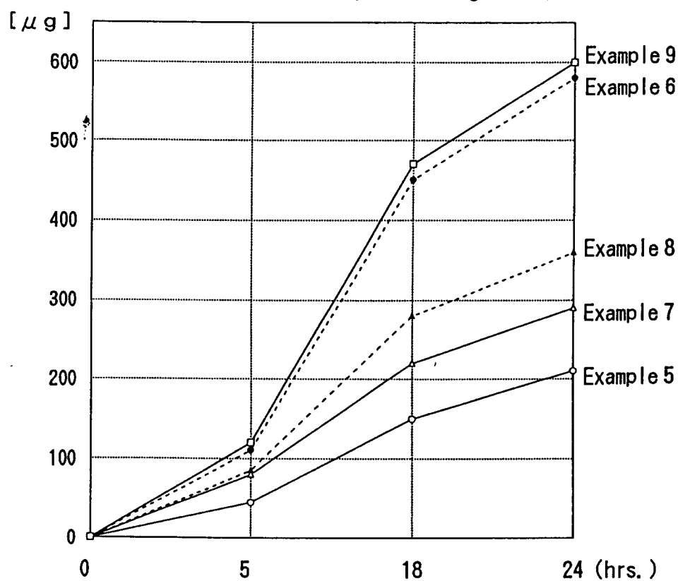
Fig. 3 Permeation Test (3-ketodesogestrel)
