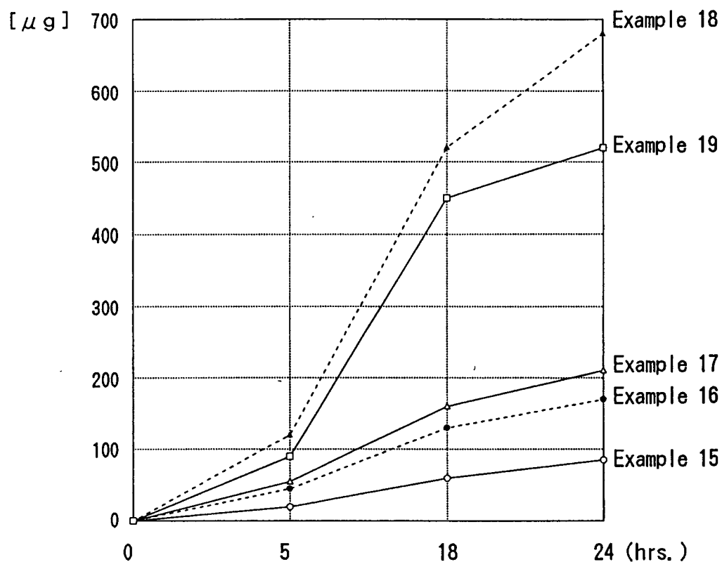
Fig. 5 Permeation Test (3-ketodesogestrel)
