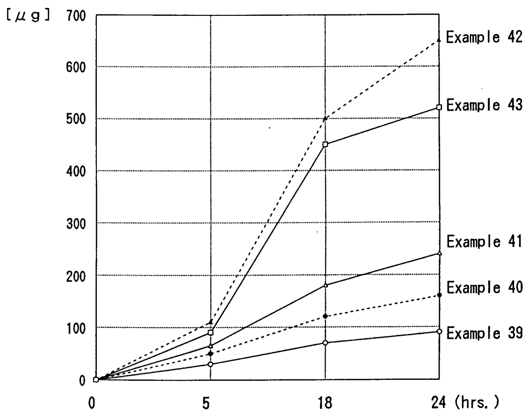
Fig. 1 6 Permeation Test (3-ketodesogestrel)
