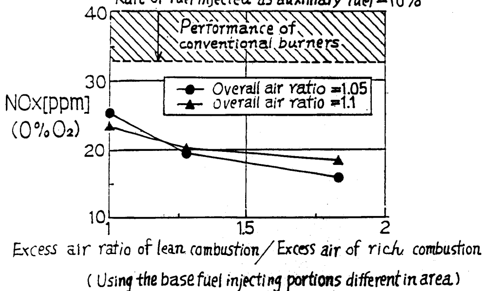
FIG.36 Combustion rate = 45 \times 10^4 [kcal/h] Flow velocity ratio (air/fuel) = 0.3 Area of the air injecting portion for forming annular air flow = 0.16 Rate of fuel injected as auxiliary fuel = 10%
