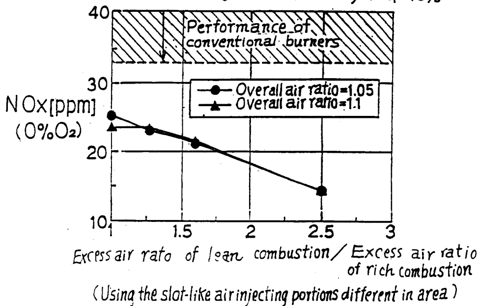
FIG.35 Combustion rate = 45 \times 10^4 [kcal/h] Flow velocity ratio (air/fuel) = 0.3 Area of the air injecting portion for forming annular air flow = 0.16 Rate of fuel injected as auxiliary fuel = 10%
