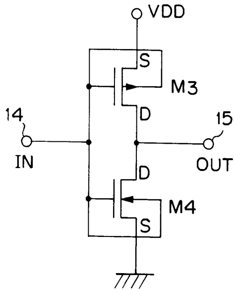
FIG. 4 (PRIOR ART)
