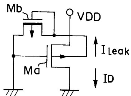
FIG.13C (PRESENT INVENTION)
