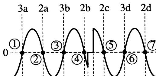
FIG. 6(b)(1) TRACKING ERROR SIGNAL (a)
