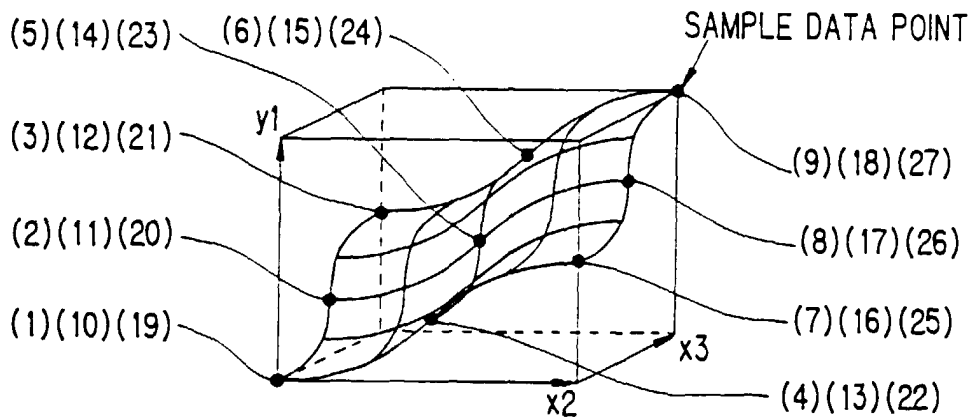
(b) FUNCTION REPRESENTED BY x_2 and x_3
