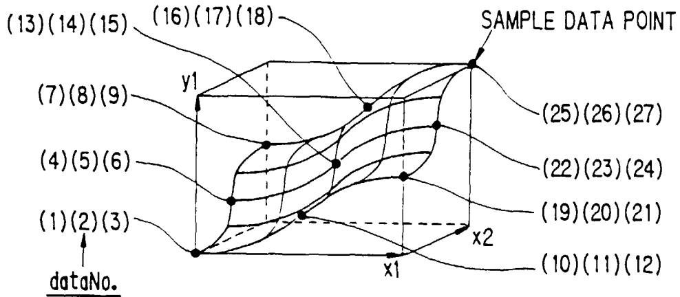
(a) FUNCTION REPRESENTED BY x_1 and x_2
