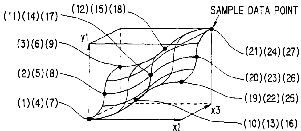
(c) FUNCTION REPRESENTED BY x_1 and x_3
