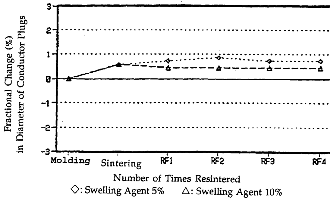
Figure 7 Consolidation Stability of Plug After Resintering
