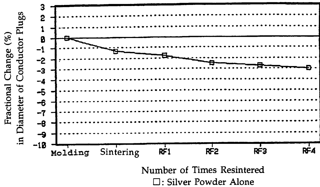
Figure 8 Consolidation Stability of Plug After Resintering
