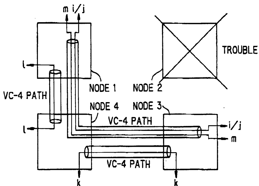
FIG.3 PRIOR ART
