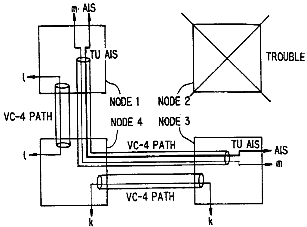
FIG.6 PRIOR ART
