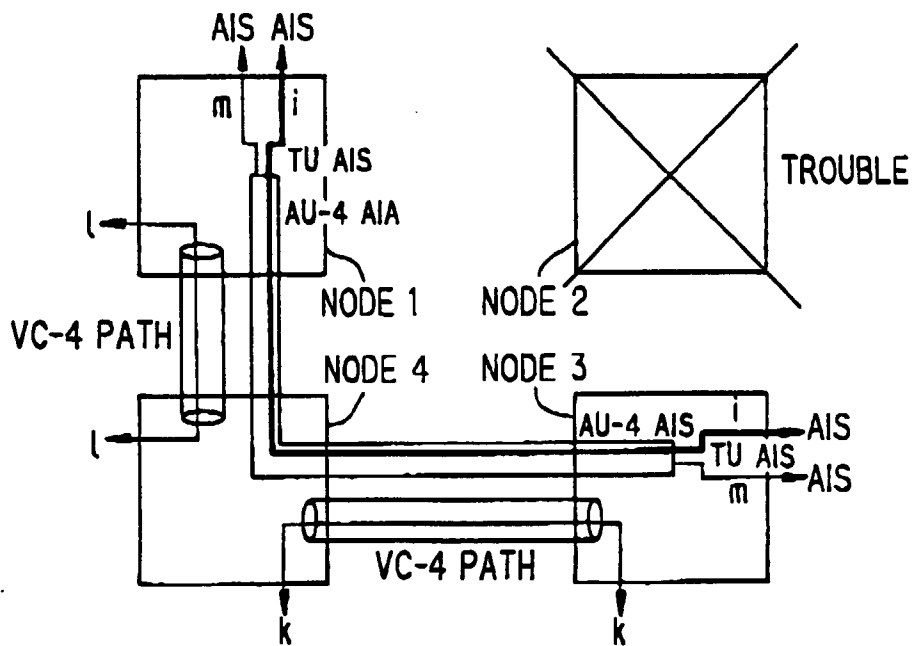
FIG.5 PRIOR ART
