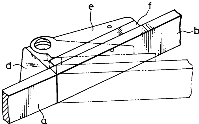
FIG. 10 PRIOR ART
