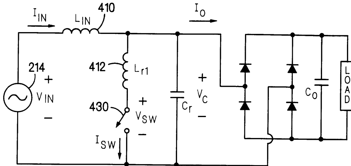
FIG. 28 (PRIOR ART)
