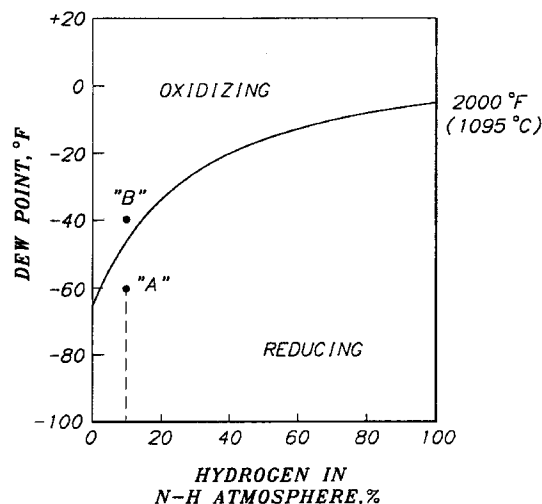
FIG. 1 OXIDATION-REDUCTION DIAGRAM FOR A TYPICAL STAINLESS STEEL
