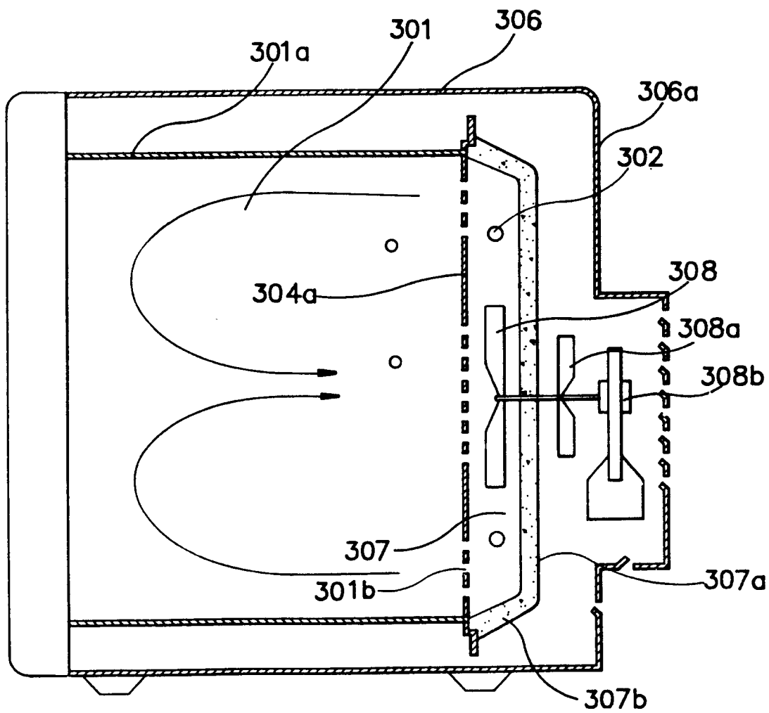
FIG. 10 (Prior Art)
