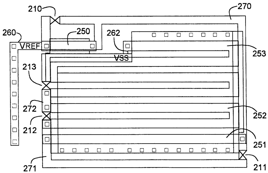
FIG. 10 PRIOR ART
