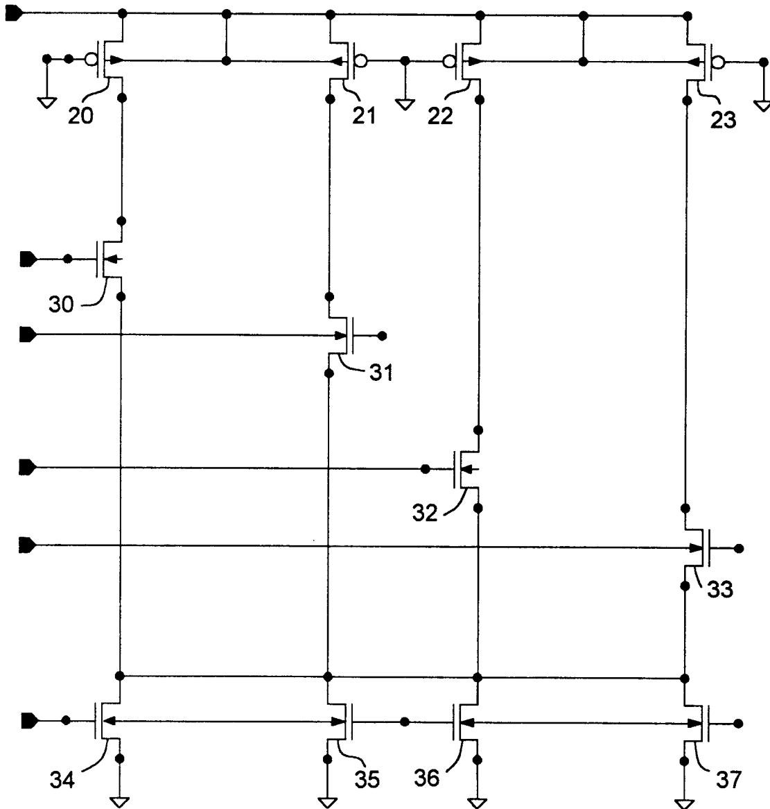
FIG. 2 PRIOR ART
