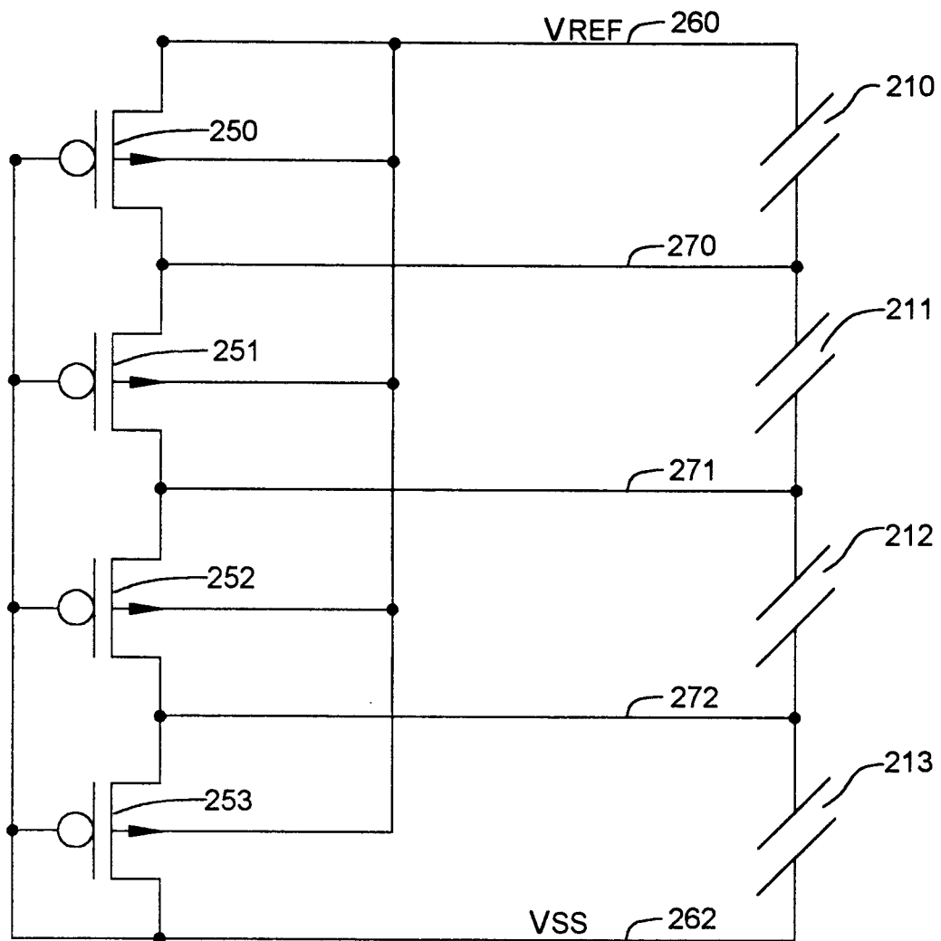
FIG. 11 PRIOR ART
