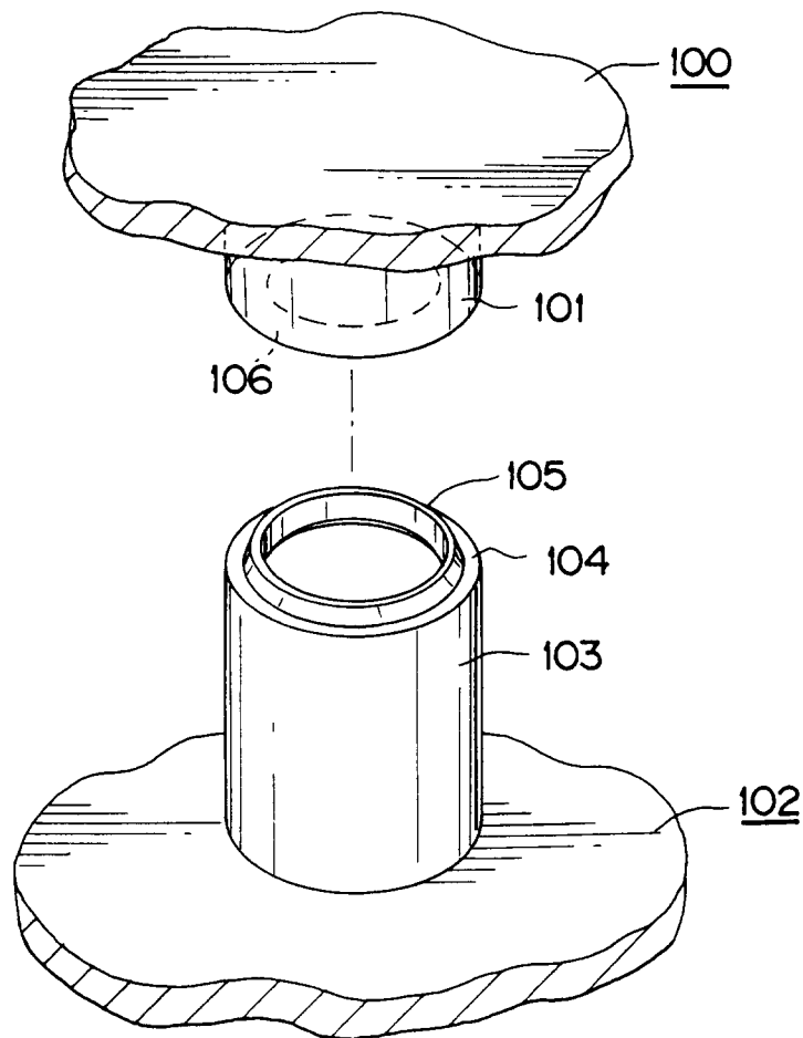
FIG.2 (PRIOR ART)
