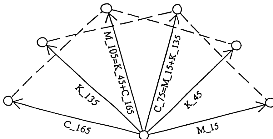
Figure 6: Interaction of three rasters at 15, 45 and 75 degrees, and with identical rulings:
