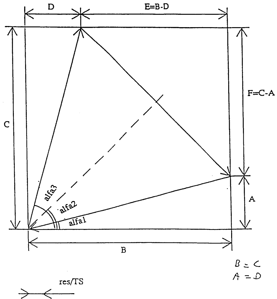
Figure 13: Vector diagram for Moire analysis.
