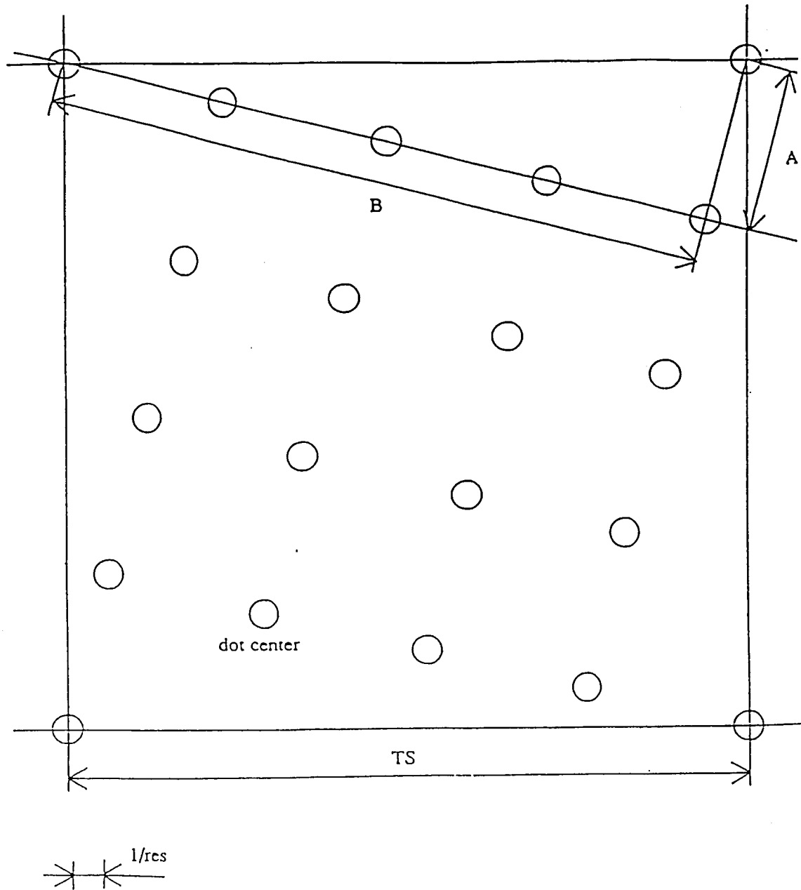
Figure 12: Geometry of a cell with preangled dots.
