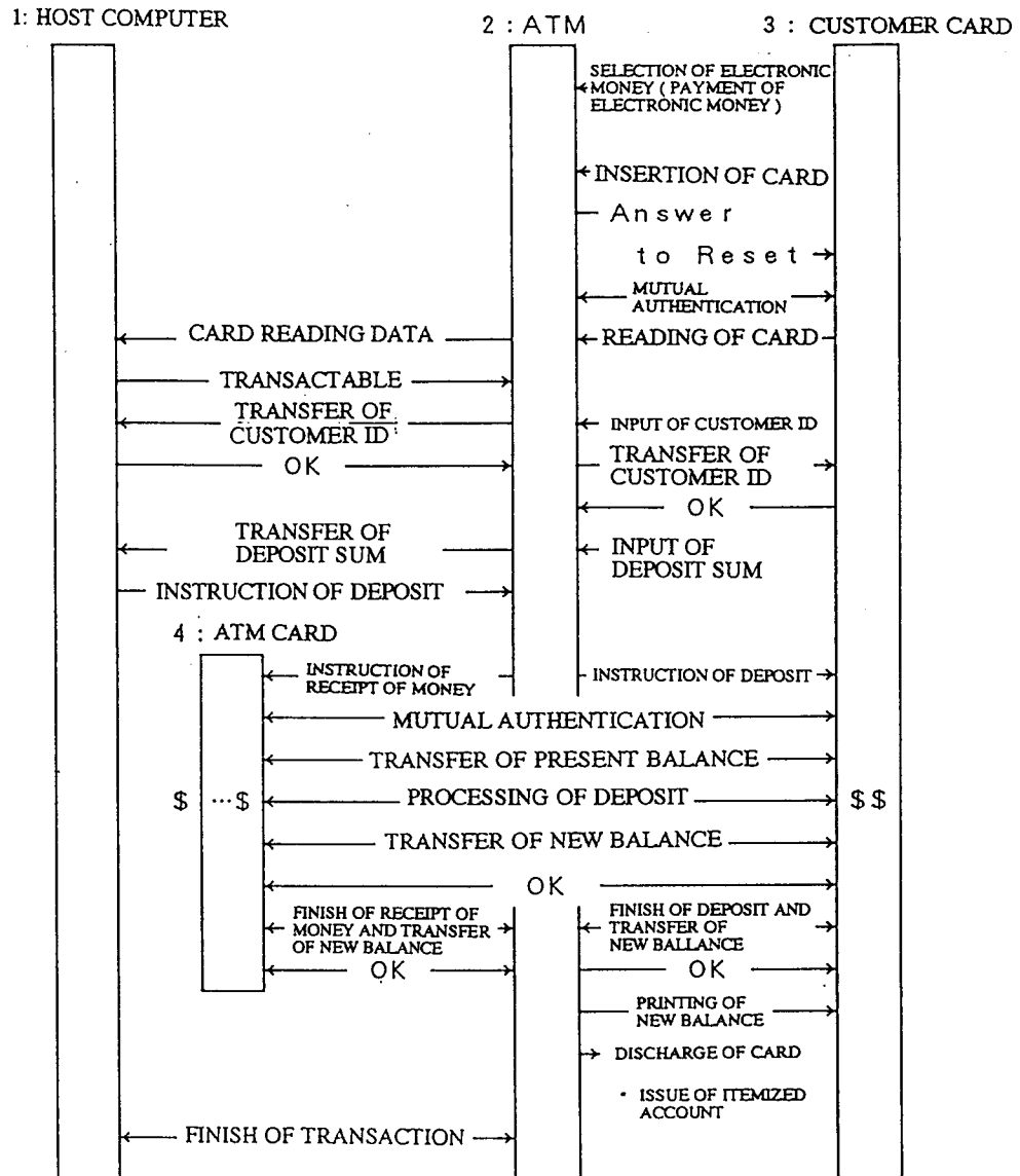
VIEW SHOWING PROCEDURES FOR TRANSACTION PROCESSING BY ELECTRONIC MONEY
