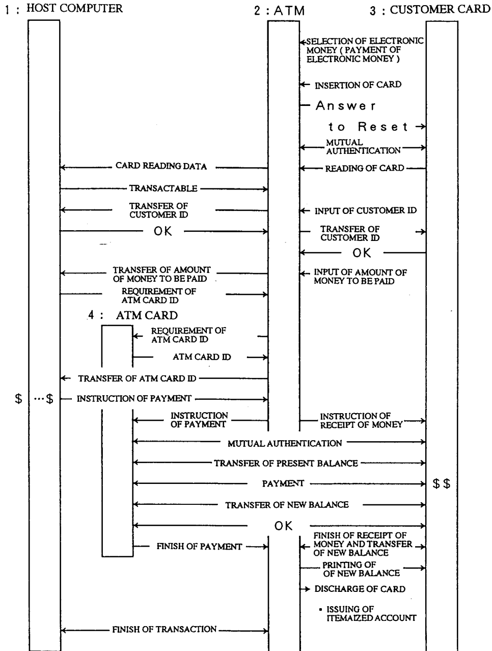
VIEW SHOWING PROCEDURES FOR TRANSACTION PROCESSING BY ELECTRONIC MEONEY
