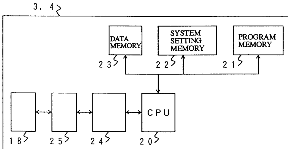
BLOCK DIAGRAM OF INSIDE OF IC CARD
