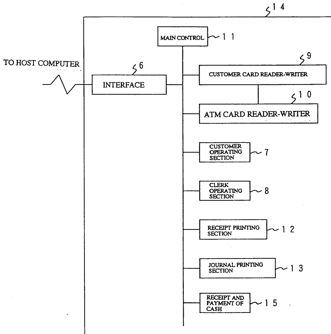
BLOCK DIAGRAM OF INSIDE OF TRANSACTION MACHINE
