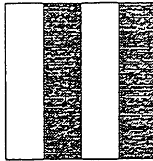
Texture image
