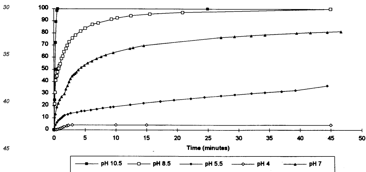
Percentage of hydrolysis of the C12 betaine ester of géraniol in function of time, at 40°C and various pH
