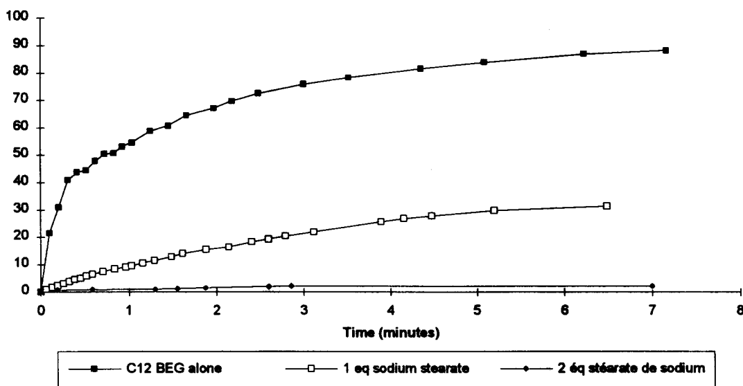
Percentage of C12 BEG hydrolysed in function of time, at pH 8.5 and 40°C constant, with various amount of sodium stearate
