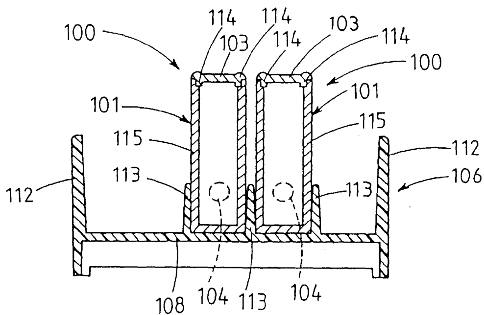
Fig.14 PRIOR ART
