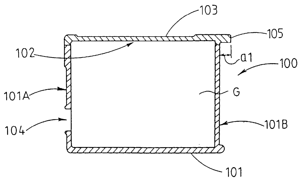
Fig.12 PRIOR ART
