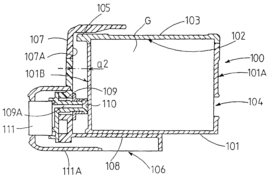
Fig.13 PRIOR ART
