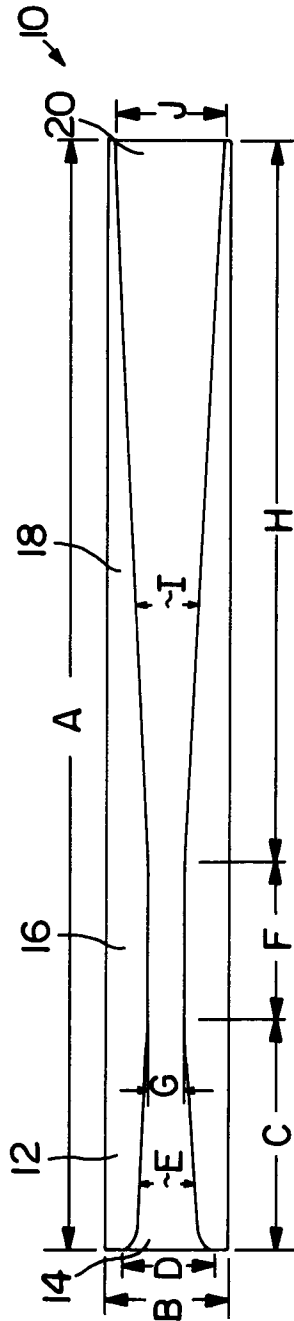
FIG. 1 PRIOR ART
