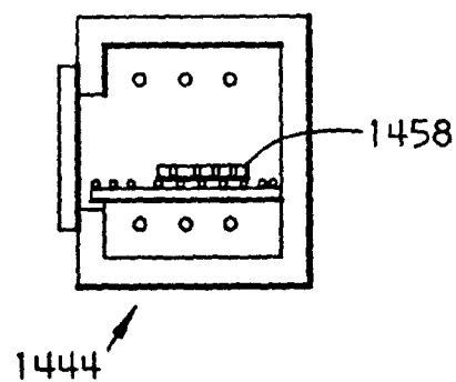
FIG. 75 (c)
