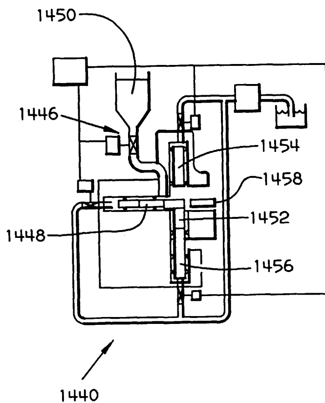
FIG. 75 (a)
