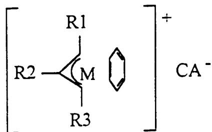
Structure IIB
