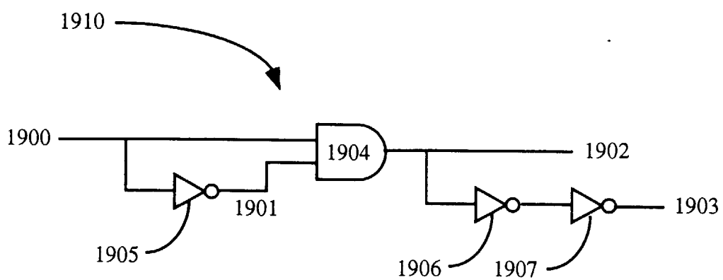
Figure 19 Prior Art
