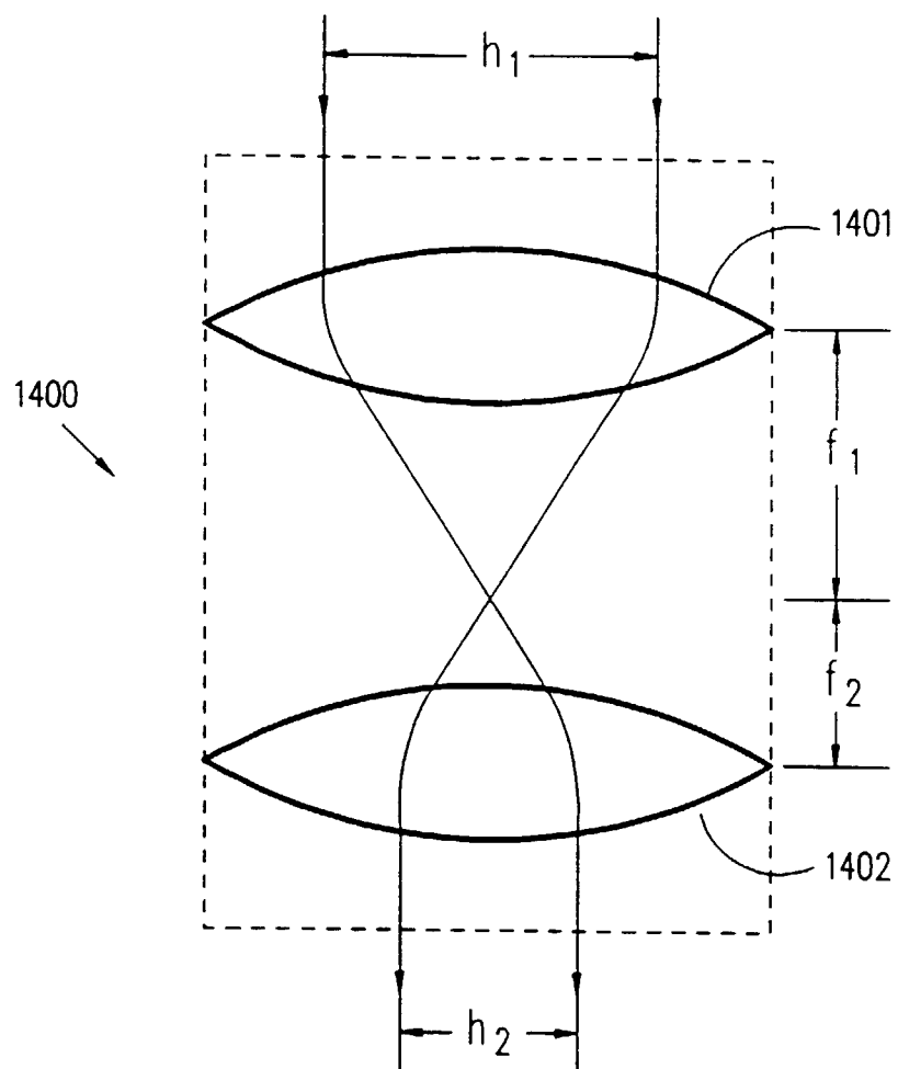
BEAM COMPRESSOR
