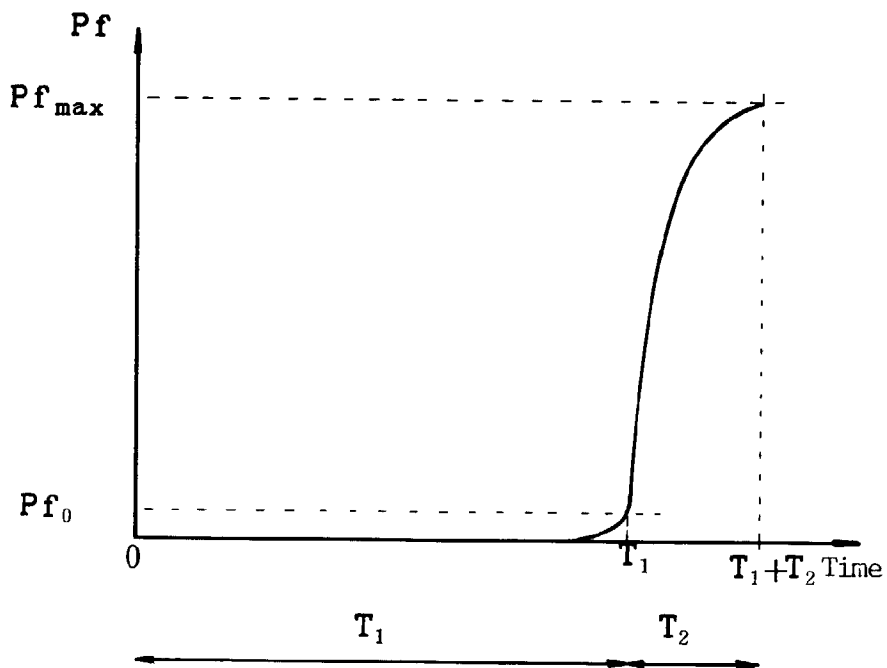
Fig.6 PRIOR ART
