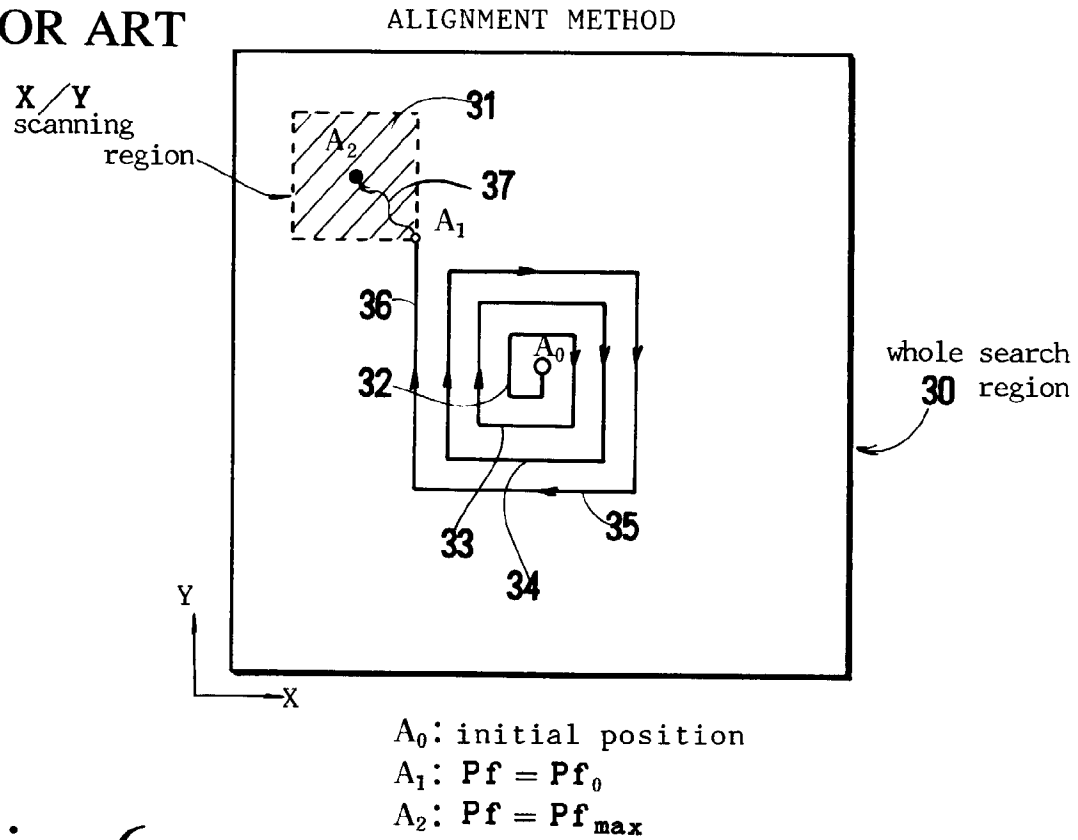
Fig.6 PRIOR ART
