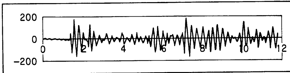
70 rpm VIBRATION WAVEFORM
