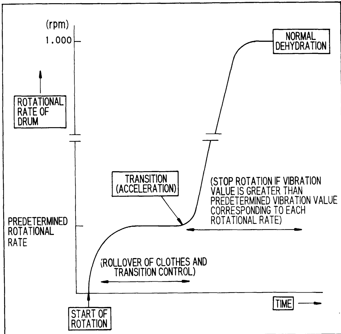
BASIC CHART OF ACCELERATION
