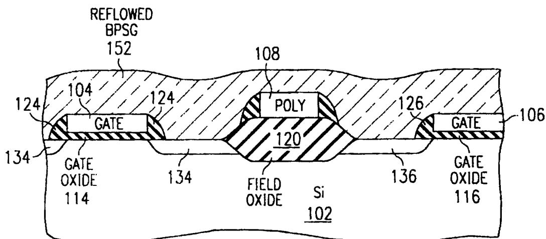
FIG. 1c (PRIOR ART)
