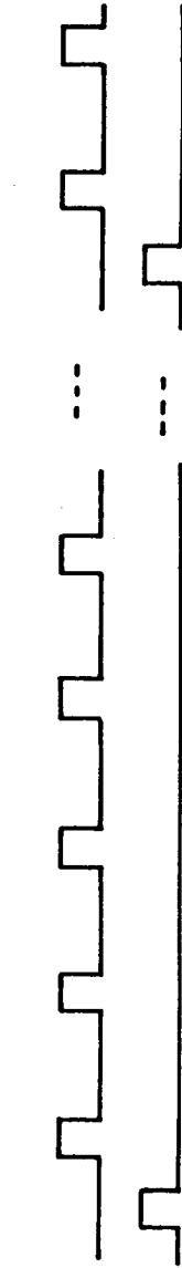
FIG. 66(b) HORIZONTAL SYNCHRONIZING HSYN
