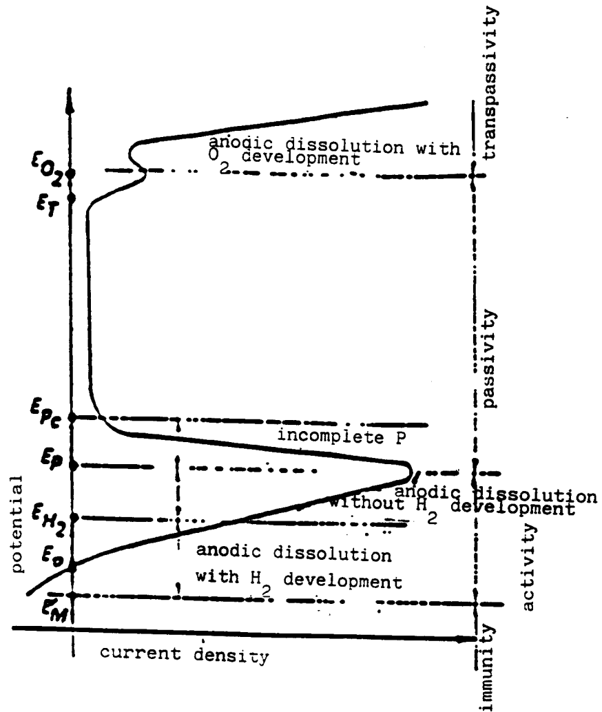
Fig.1 Typical polarization curve of stainless steel in deaerated acid solution
