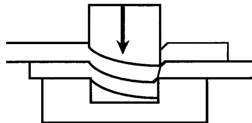
6 BONDING COMPLETION
