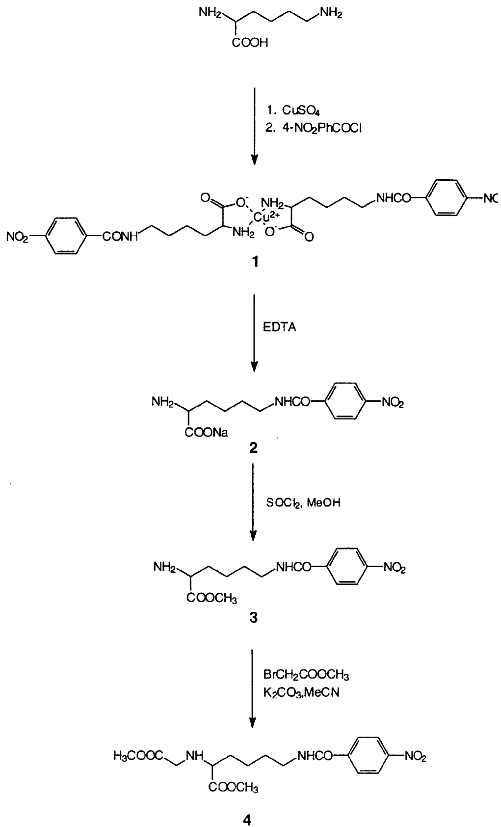
SCHEME 1.
