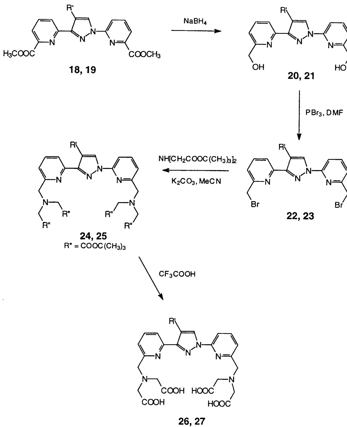
SCHEME 5.
