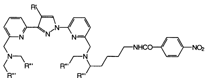
28, 29 \text{R}''' = \text{COOCH}_3
