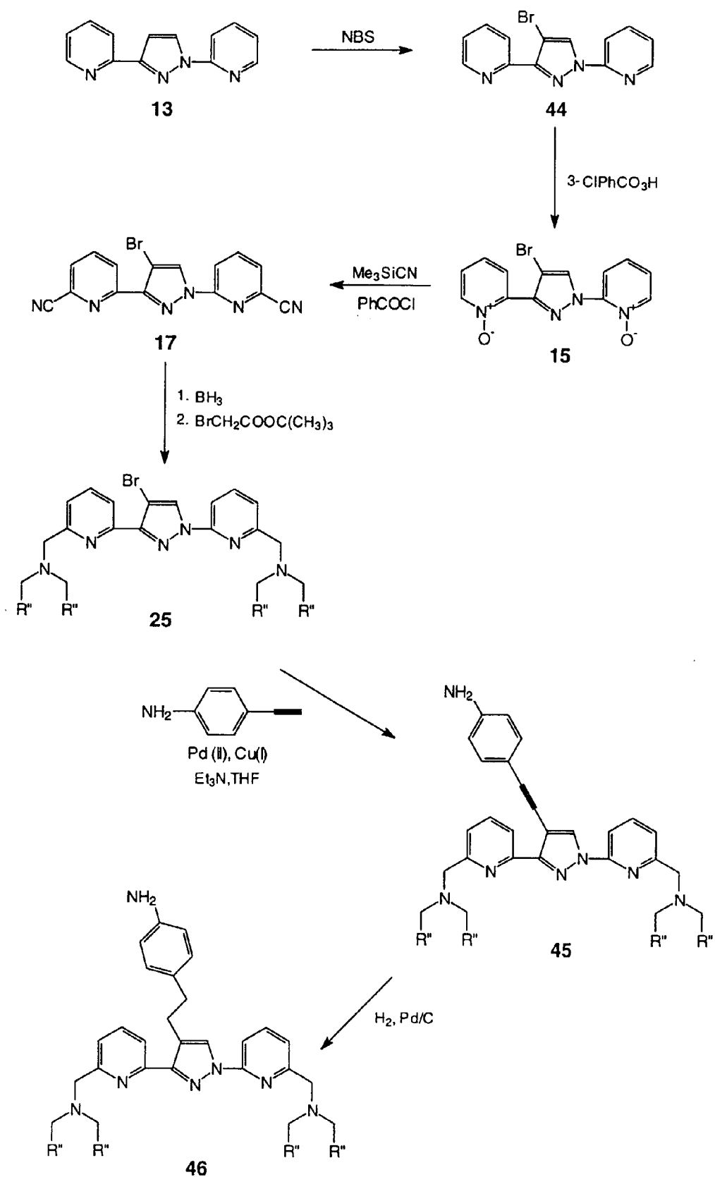
SCHEME 10.
