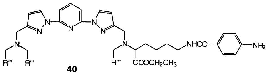
SCHEME 8.
