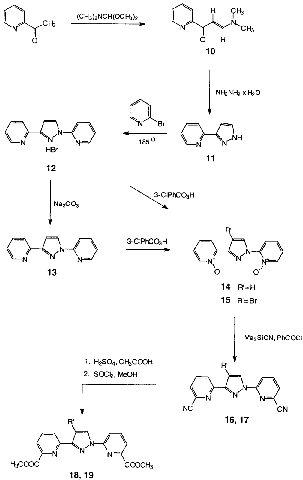
SCHEME 4.
