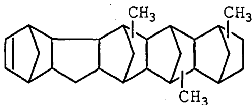
Trimethyl-substituted- nonacyclo- [10.9.1.14,7.113,20. 115,18.03,8.02,10.012,21. 014,19]-5-pentacosene
