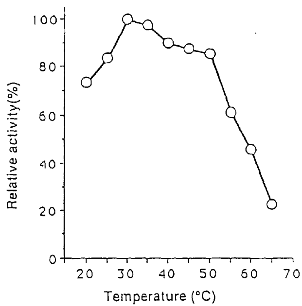
Effect of temperature on yeast ADH activity
