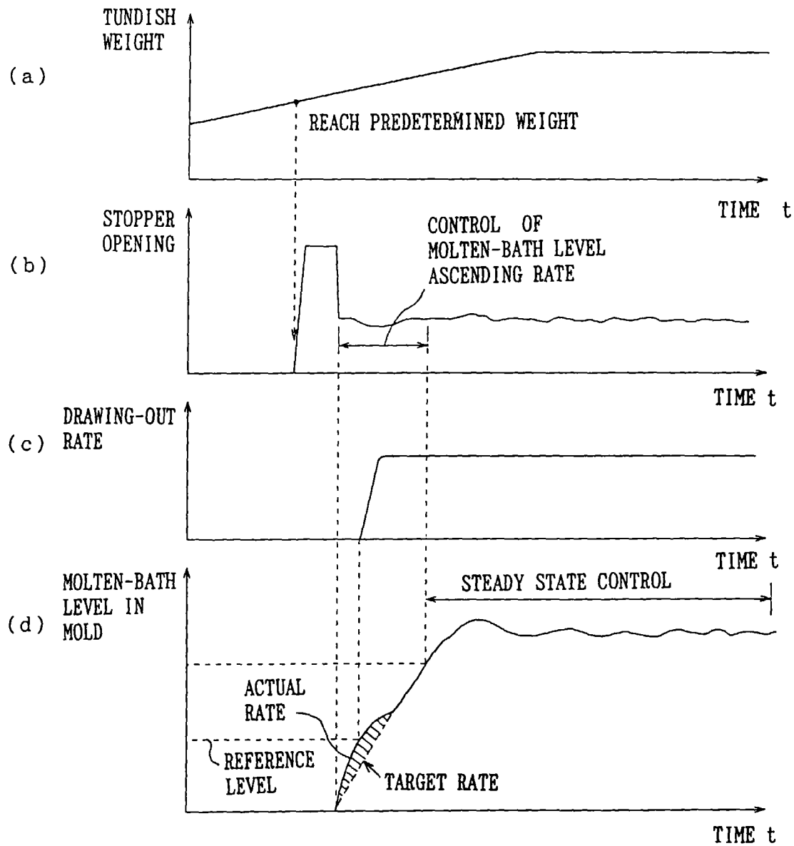
CONTROL CHART
