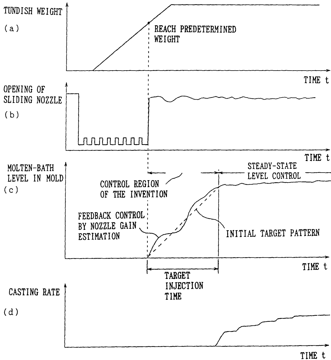
CONTROL CHART
