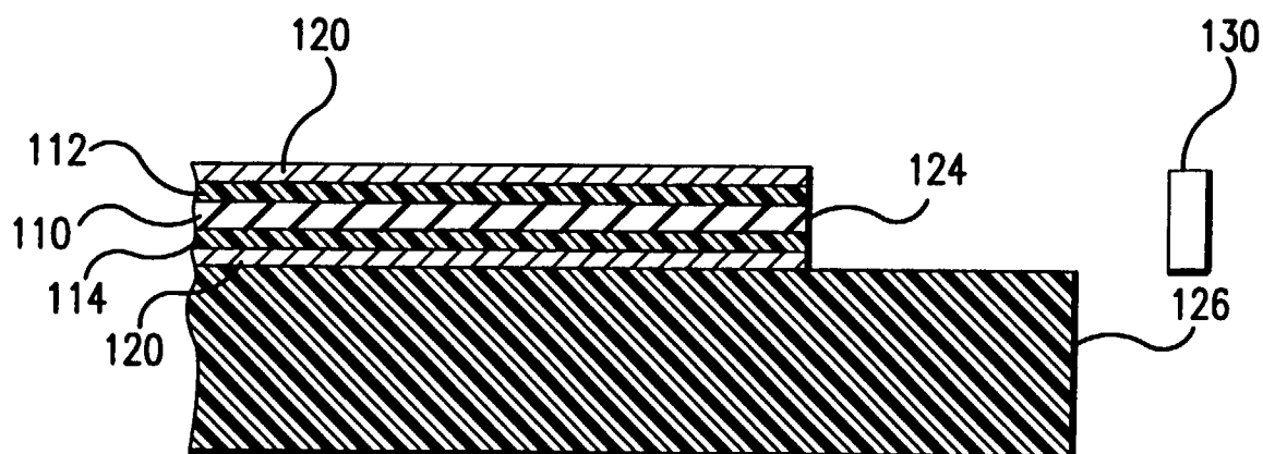
FIG.1 PRIOR ART
