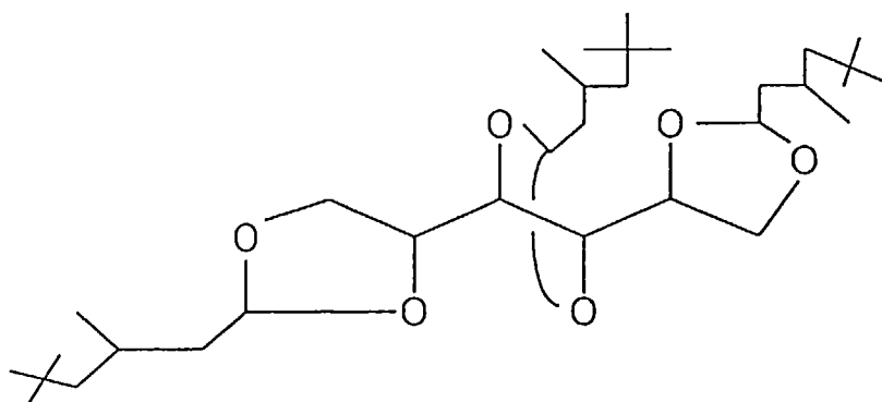
(3) 1,2:3,4:5,6-tri-O-(3,5,5-trimethylhexylidene)sorbitol
