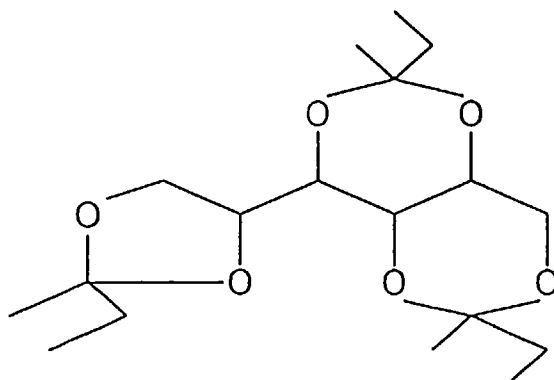
(6) 1,3:2,4:5,6-tri-O-(1-methylpropylidene)sorbitol
