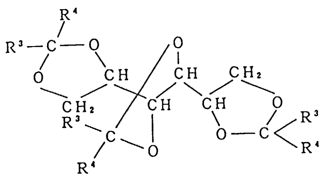
(IIIa)
