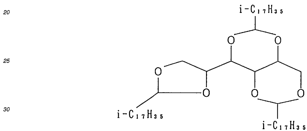
(12) 1.3:2.4:5.6-tri-O-(isooctadecylidene)sorbitol
