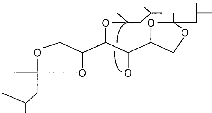
(7) 1,2:3,4:5,6-tri-O-(1,3-dimethylbutylidene)sorbitol
