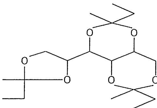
(18) 1,3:2,4:5,6-tri-O-(1-methylpropylidene)mannitol
