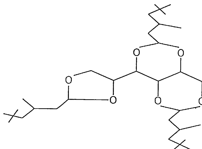
(4) 1,3:2,4:5,6-tri-O-(3,5,5-trimethylhexylidene)sorbitol
