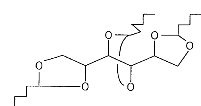
(9) 1,2:3,4:5,6-tri-O-(hexylidene)sorbitol
