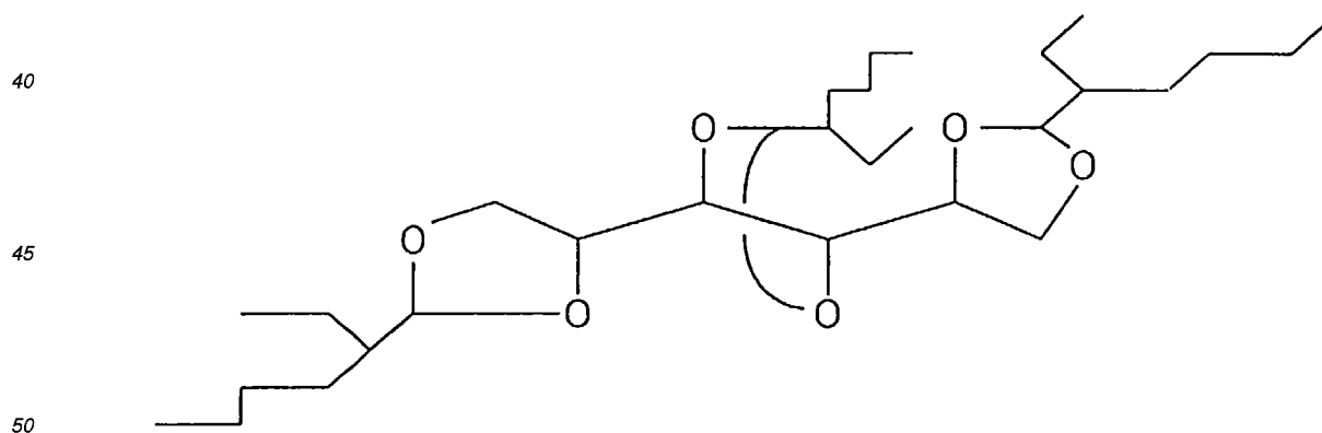
(13) 1.2:3.4:5.6-tri-O-(2-ethylhexylidene)sorbitol
