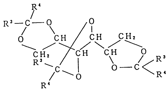
(IIIa)
