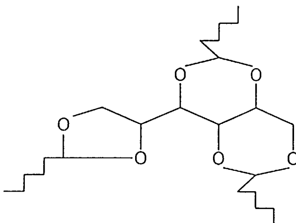
(10) 1,3:2,4:5,6-tri-O-(hexylidene)sorbitol
