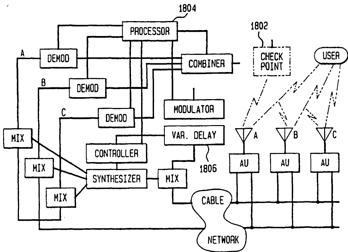
FIG. 18 TIME CALIBRATION FOR DISTRIBUTED ANTENNA IMPLEMENTATION
