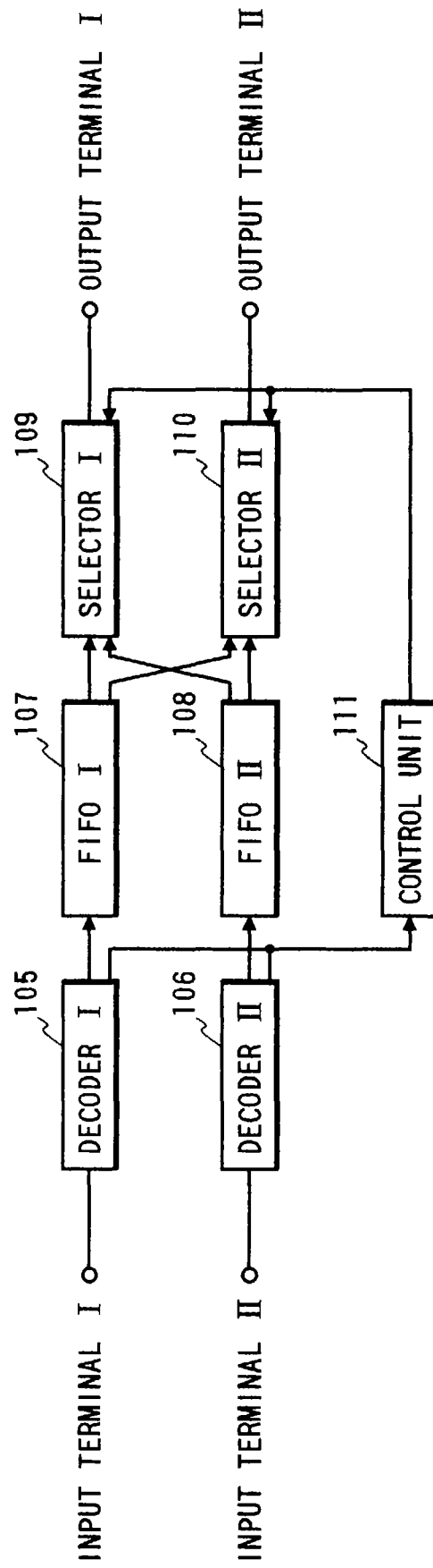
FIG. 17 PRIOR ART
