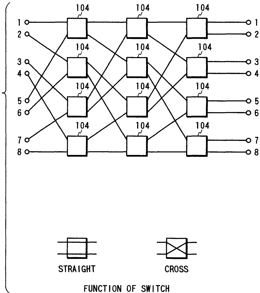
FIG. 16 PRIOR ART
