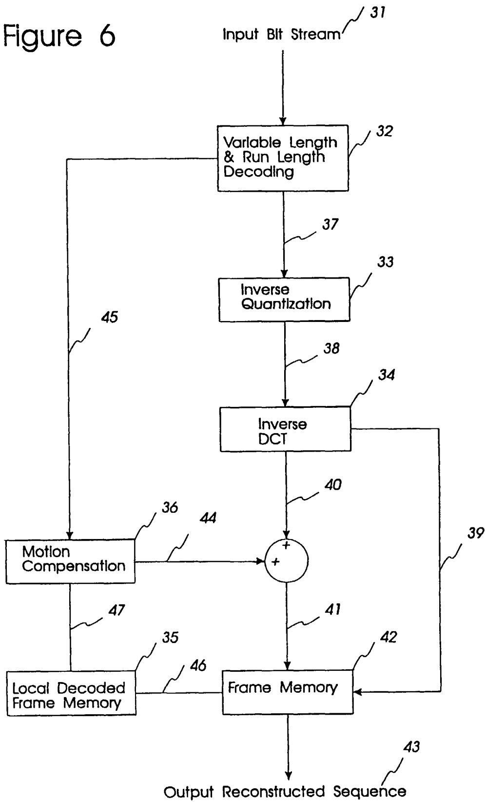
Decoder Block Diagram
