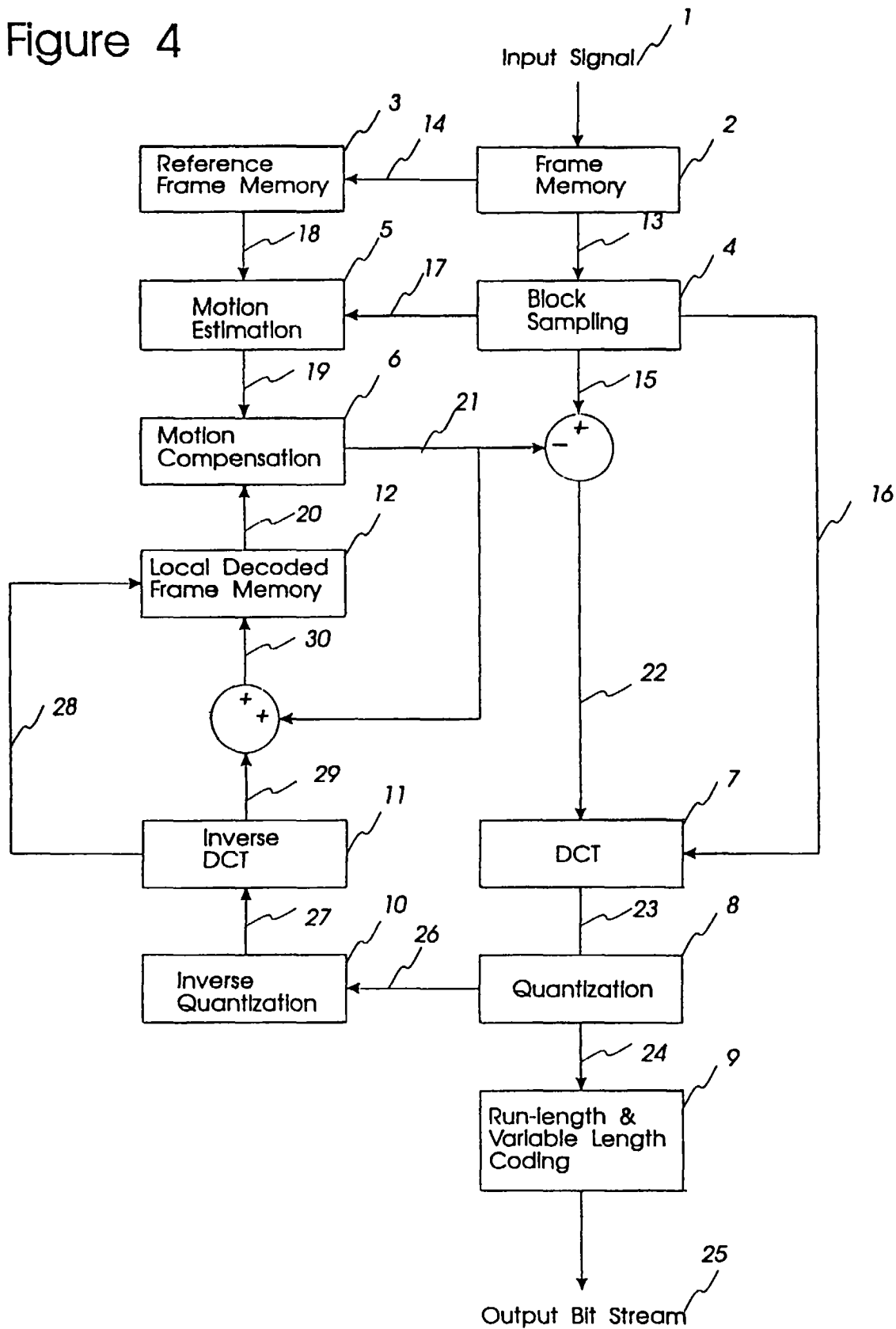
Encoder Block Diagram
