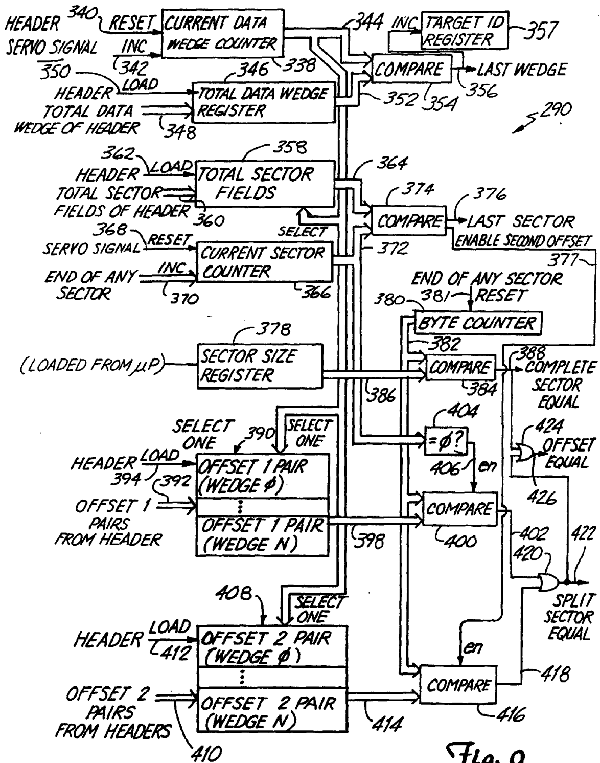
MULTIPLE DATA WEDGE PER HEADER METHOD 1 BLOCK DIAGRAM
