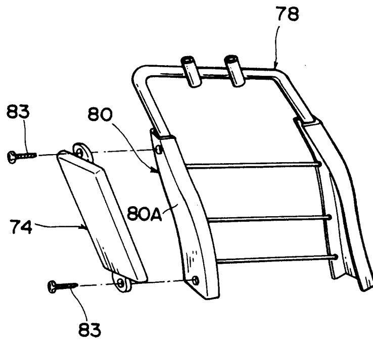
FIG. 8 PRIOR ART
