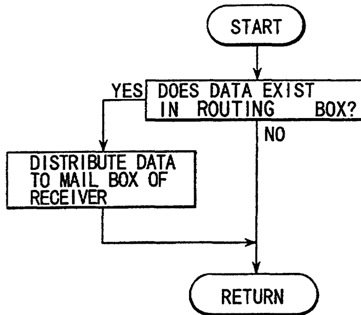
MAIL DISTRIBUTION PROGRAM
