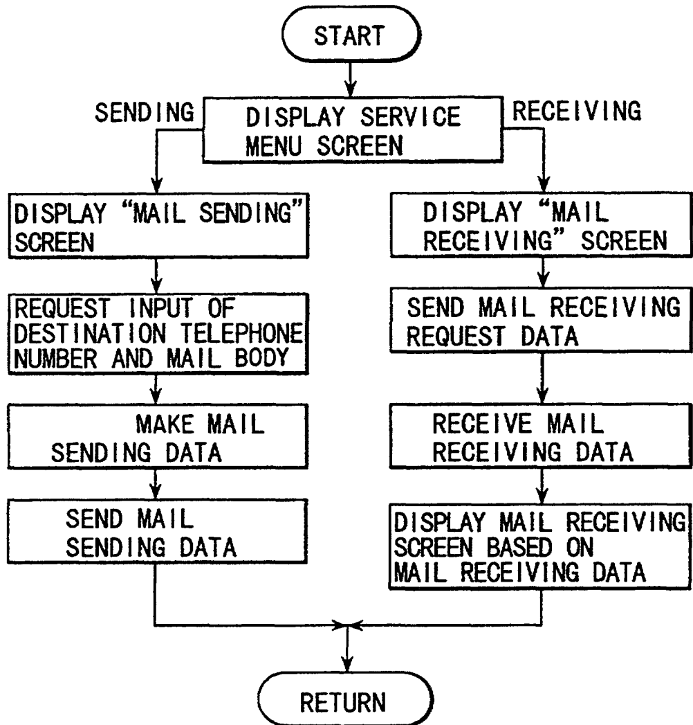
FLOWCHART OF INTERACTIVE TV
