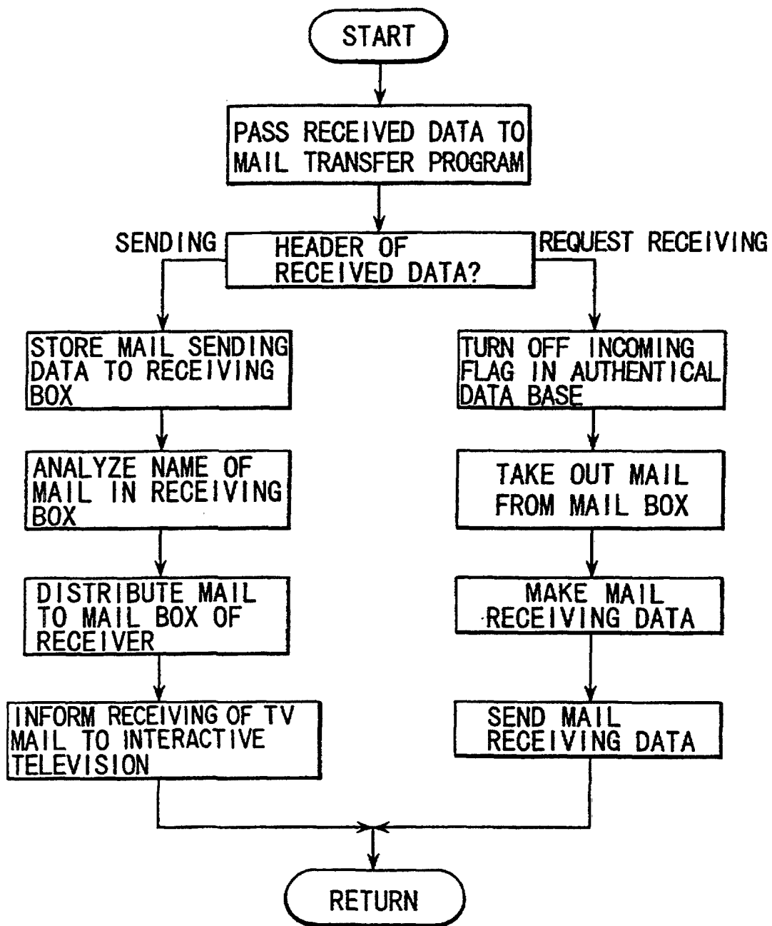
FLOWCHART OF CENTER RESPONSE SERVER
