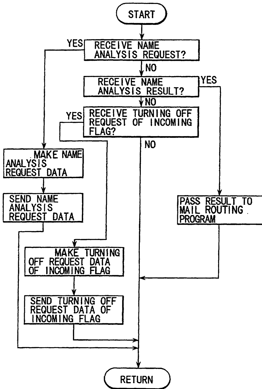
NAME ANALYSIS CLIENT PROGRAM
