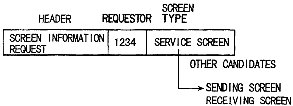
SCREEN INFORMATION REQUEST DATA
