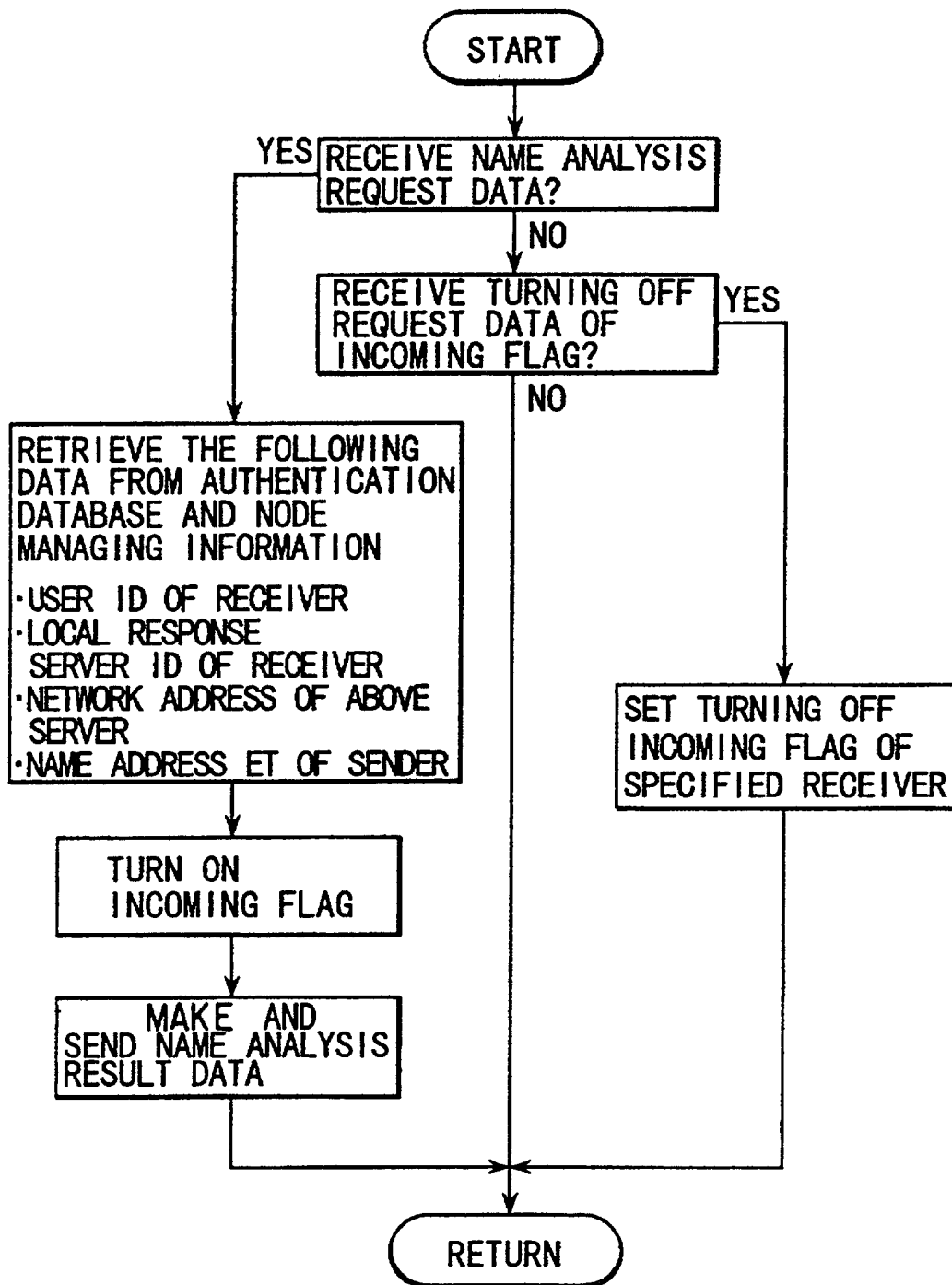
NAME ANALYSIS SERVER PROGRAM
