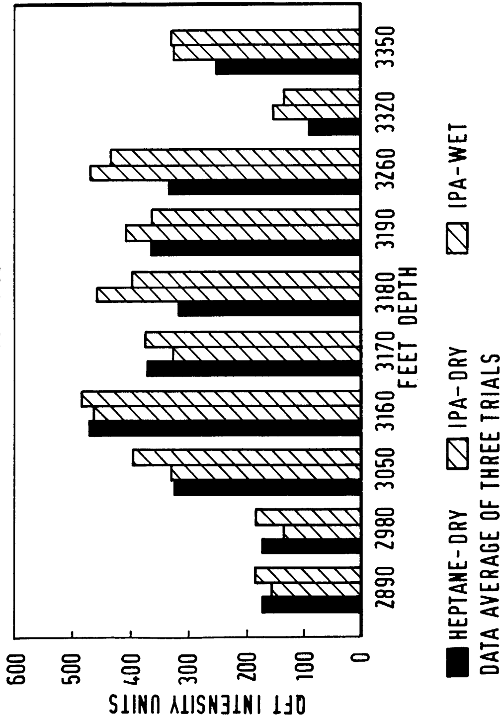
FIG. 6 SOLVENT FOR WET CUTTINGS DRILL CUTTINGS
